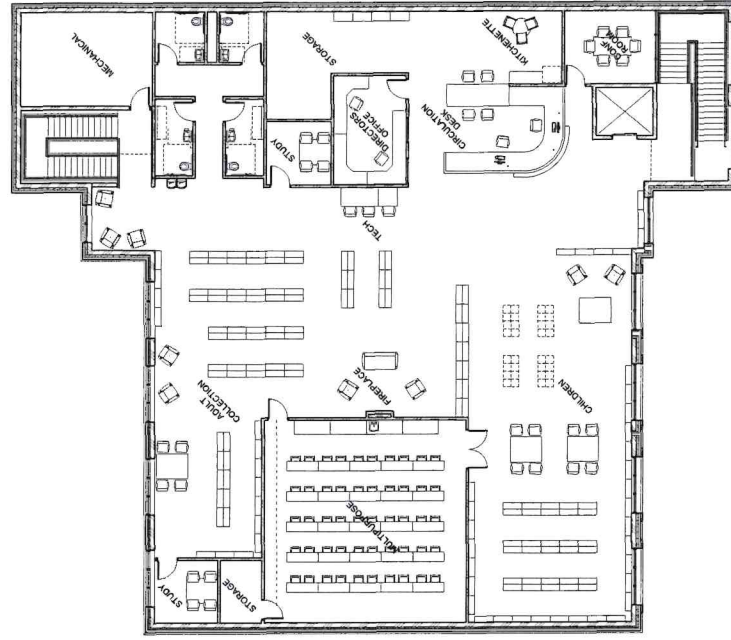
2 UPPER FLOOR PLAN SCALE: 1/8" = 1'-0"
